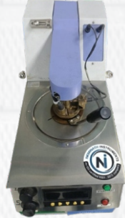
Pensky Marten - Semi automatic model ASTM D93
