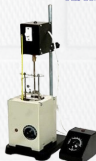
Softening point apparatus ASTM D36
