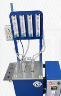
Oxidation Stability of Lubricating oil BS 2000
