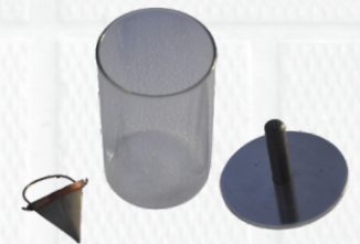
Oil Separation from Lubricating grease - Conical Sieve method ASTM D6184
