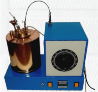
Abel's Flash point apparatus with Voltage Variac and Motorised Stirrer IP-170, IS 1448 (P-20)
